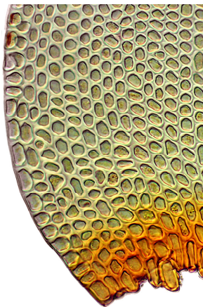
leaf basal angle 50 \mu m
