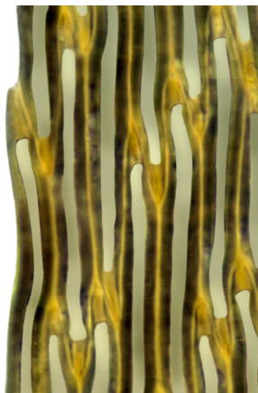
margin midleaf 10 \mu m
