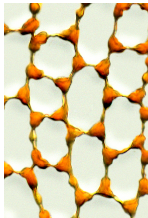
trigonous capsule wall cells 20 \mu m
