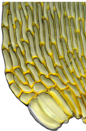
leaf basal angle 10 \mu m
