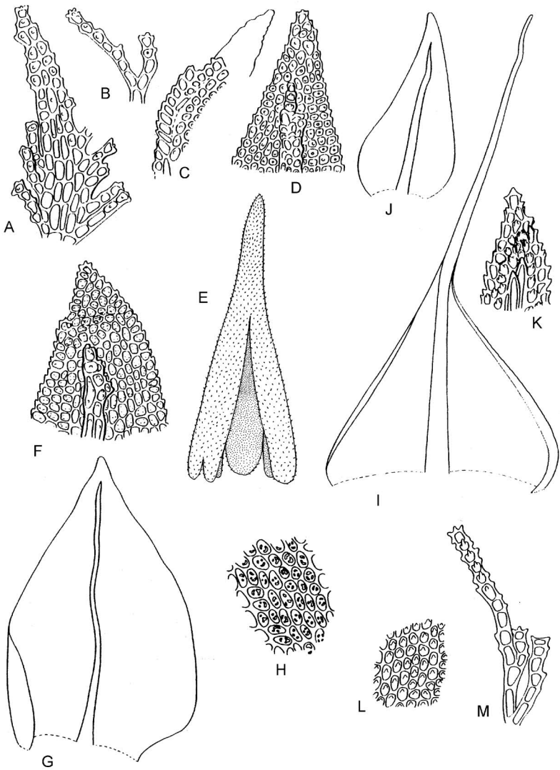
Thuidium. A–E , T. plumulosum . A , pseudoparaphyllium; B , paraphyllium; C , crest on branch leaf in side view; D , apex of branch leaf; E , calyptra (A–E, C.Kalkman BW 3534, L). F , T. laeviusculum ; apex of branch leaf (E.Whitehouse 29378, MO). G, H , T. subglaucinum . G , stem leaf; H , areolation of branch leaf (G, H, H.Streimann 1768, L). I–M , T. cymbifolium . I , stem leaf; J , branch leaf; K , apex of branch leaf; L , areolation of branch leaf; M , paraphyllia (I–M, E.F.Constable NSW 11064).
